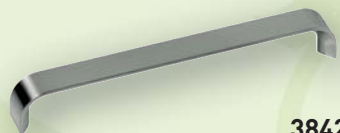
3842 Total Length - 201/20mm Centres - 192mm Finish - Brushed Nickel
